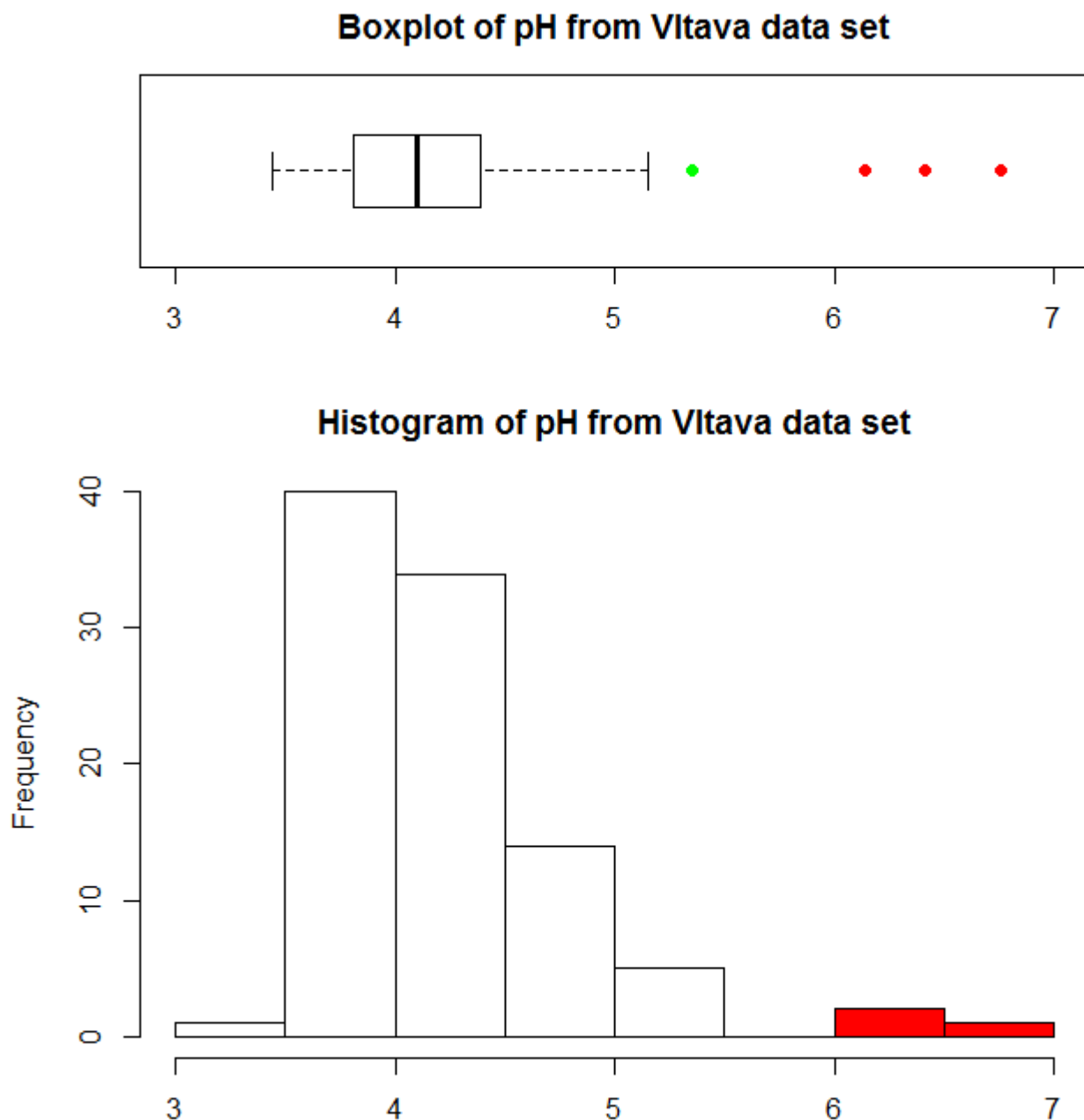
Figure 2: Boxplot (above) and histogram (below) of soil pH values from Vltava river valley dataset.
